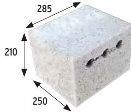
B-33 External corner piece
