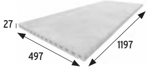
Borde monocompact 120 Monocompact edge 120
