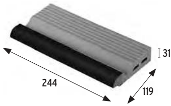
Finnish miter joint internal corner
