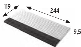
Canto romo ranurado Bullnose int. corner
