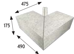
External corner piece
