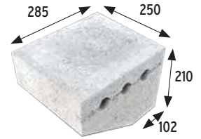
B-33 Niche piece
