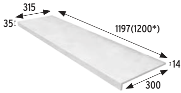
Straight stair-tread 120
