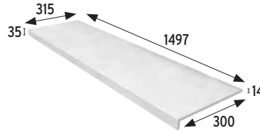
Straight stair-tread 150
