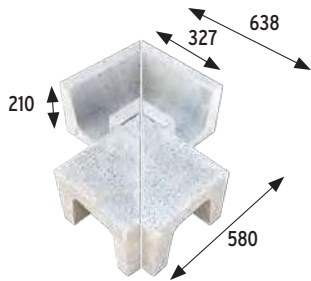
B-33 Internal corner piece
